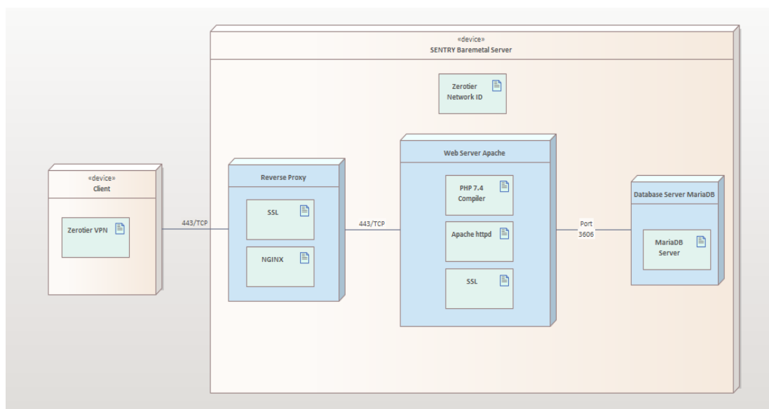
Gambar 4. Deployment Diagram
