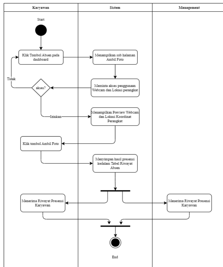
Gambar 2. Activity Diagram Presensi Karyawan
